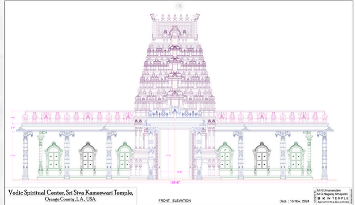
Front elevation plan
